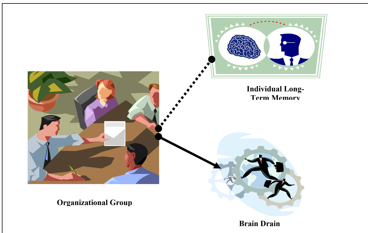
Figure 1: Knowledge Reserve
